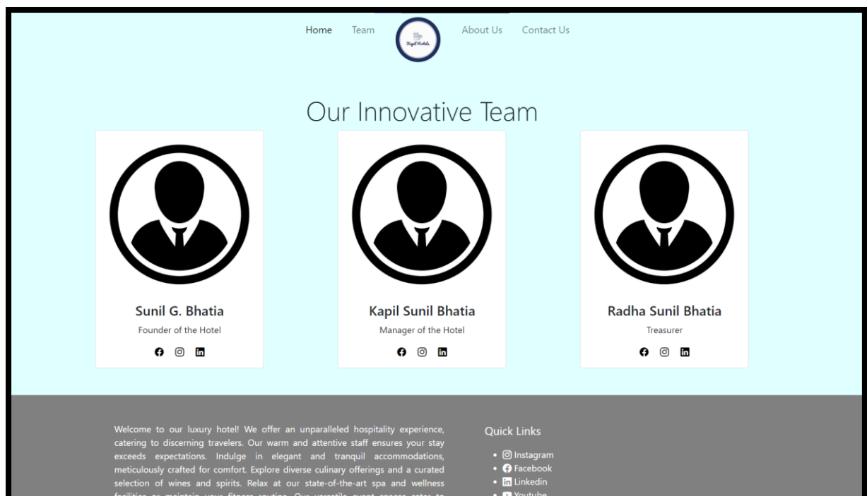
Fig 2: Teams Page
