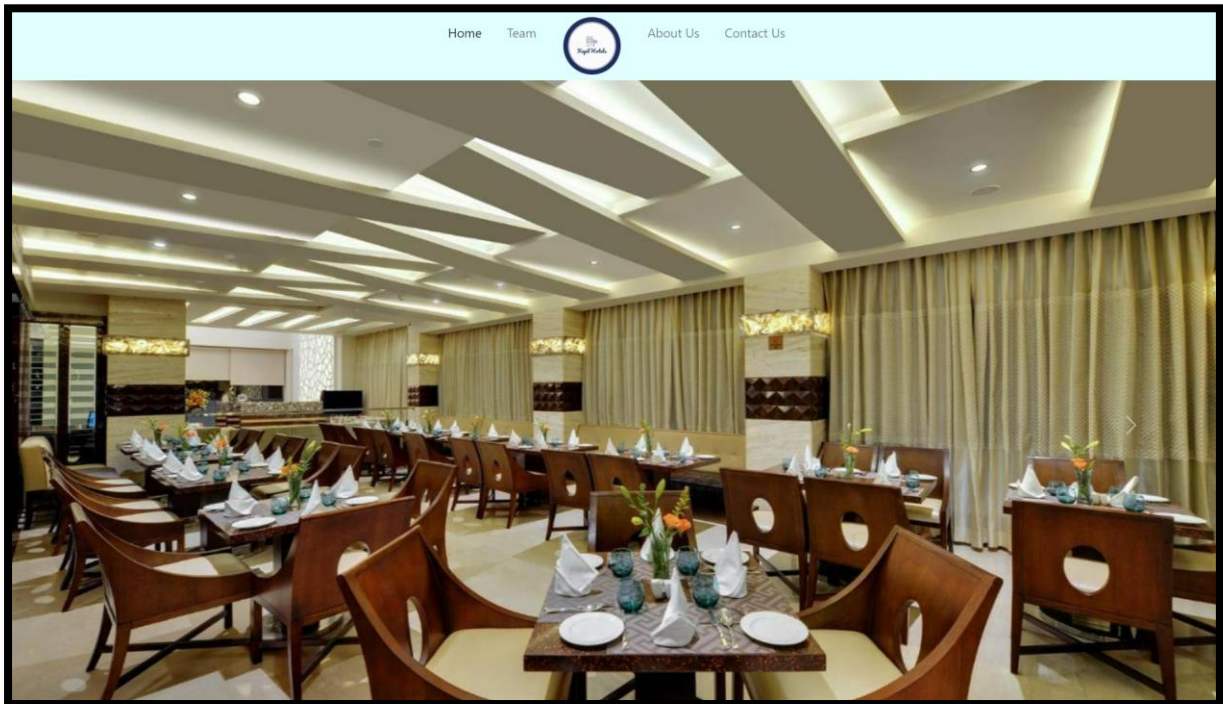
Fig 1.1: Home Page
